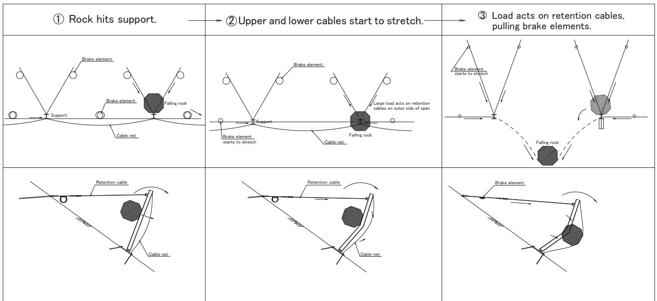
System behavior when falling rock directly hits support
