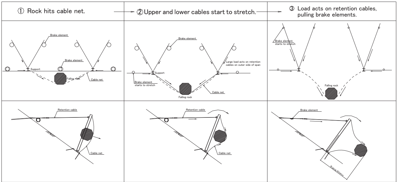
System behavior when falling rock is captured between supports
